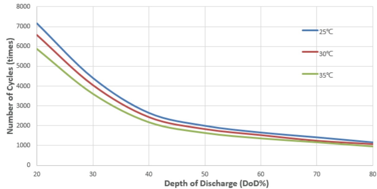
FTC-C battery cycles lifetimes VS depth of discharge
