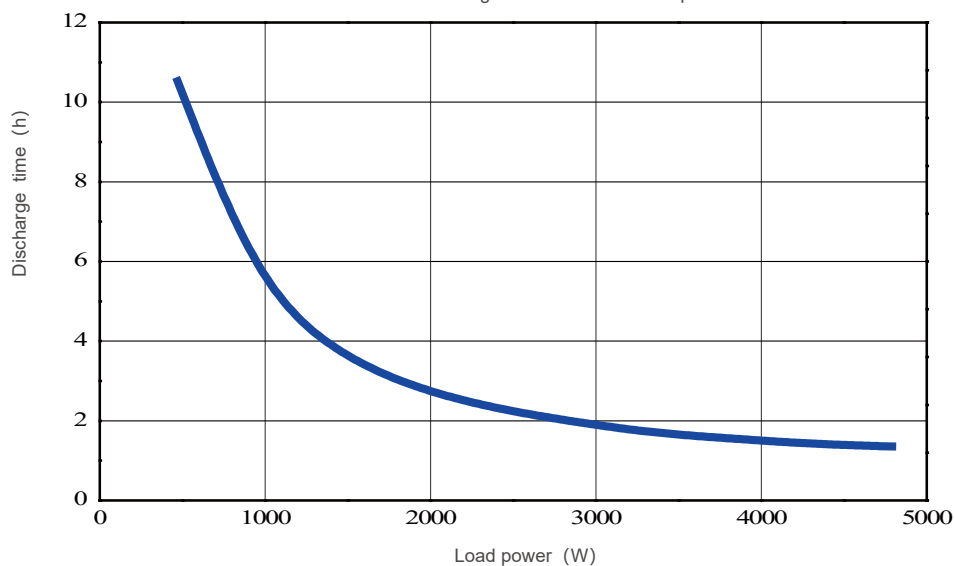
SDA10-48150 Discharge time at different load power
